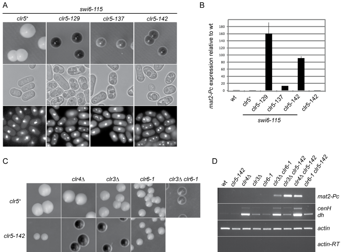
Figure 2. Clr5 acts in the same pathway as the HDAC Clr6 and represses mat2-P independently of Swi6, Clr3, and Clr4. (A) SPK29 and mutants obtained by insertional mutagenesis in SPK29. Colonies formed on MSA sporulation plates were stained with iodine (top panels). All strains contain the mat1-Msmt-0 cassette hence like in Figure 1 staining correlates with mat2-P expression. Cells from the same strains were imaged by DIC (middle panels) or fluorescence microscopy following DAPI staining (bottom panels). Spores are visible in DIC and as multiple DAPI-stained nuclei in clr5-129 swi6-115 (SPK129), clr5-137 swi6-115 (SPK137), and clr5-142 swi6-115 (SPK142) double mutants but not in the swi6-115 (SPK29) unmutagenized strain. (B) Real-time RT-PCR quantification of mat2-Pc transcript presented as mat2-Pc /actin ratios normalized to wild-type levels. RNA was prepared from cells propagated for 5 hours in ME. Strains from left to right: PG1789, SPK29, SPK129, SPK137, SPK142 and SPK368. (C) Epistasis analysis. mat1-Msmt-0 colonies formed on MSA sporulation plates were stained with iodine. Full derepression of mat2-P is observed when defective clr5 and clr3 or clr4 alleles are combined indicating Clr5 acts in a pathway distinct from Clr3 and Clr4. In contrast, no cumulative effect is seen when combining defective clr5 and clr6 alleles indicating Clr5 and Clr6 act in the same pathway, at least for their effects in the mating-type region. Top panel: PG1789, SPK450, PG3564, SP1240, PG3577. Bottom panel: SPK368, SPK447, SPK415, SPK493. (D) mat2-Pc and transcripts with centromere homology originating from centromeres ( dh ) or the mating-type region ( cenH ) were detected by RT-PCR using the same strains as in C. doi:10.1371/journal.pgen.1001268.g002
