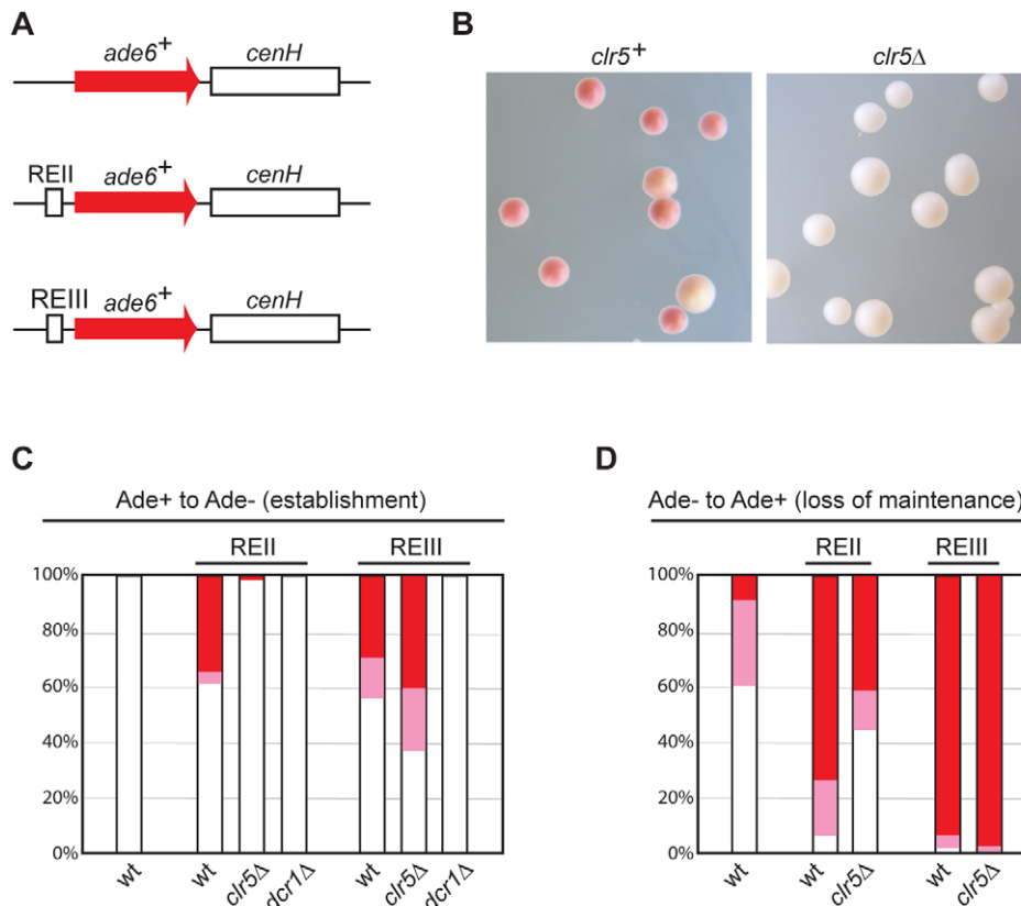
Figure 7. Clr5 mediates gene silencing at an ectopic site in an REII-dependent manner. (A) Schematic representation of constructs inserted at the ura4 locus to monitor the effects of cenH , REII, REIII, and selected trans -acting factors on ectopic silencing. (B)–(D) Silencing of the REII- ade6 + - cenH ectopic construct depends on Clr5. (B) clr5 + and clr5Δ strains with REII- ade6 + - cenH were propagated on plates poor in adenine (AA with 15 mg/l adenine). On these plates, cells in which REII- ade6 + - cenH is repressed form red or pink colonies and cells in which REII- ade6 + - cenH is expressed form white colonies. Cells from white (C) or red (D) colonies were replated on medium with a low adenine concentration and white, pink, and red colonies were counted, hereby determining the proportion of cells that had changed their epigenetic state. At least 200 colonies were counted on each plate. The ade6 + - cenH WT strain was AP2374; the REII- ade6 + - cenH strains (marked REII ) were: WT: AP2374; clr5Δ : AP2354; dcr1Δ : AP2403; the REIII- ade6 + - cenH strains (marked REIII ) were: WT: AP1665; clr5Δ : AP2346; dcr1Δ : AP2406. doi:10.1371/journal.pgen.1001268.g007
